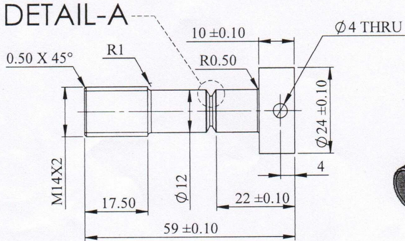
DETAIL-A SCALE 5 : 1
