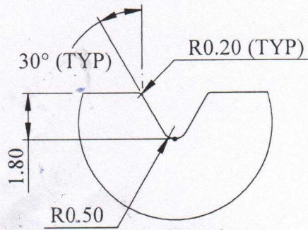
DETAIL-A SCALE 5 : 1
